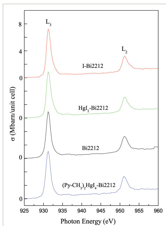
Fig. 3: Cu L_{2,3} -edge X-ray absorption spectra of I-Bi2212, \text{HgI}_2 -Bi2212, Bi2212 and (\text{Py-CH}_3)_2\text{HgI}_4 -Bi2212.
