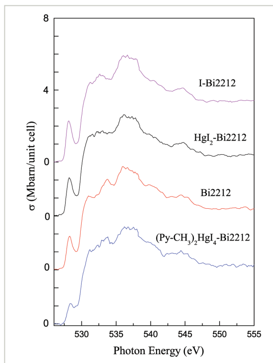
Fig. 1: O K-edge X-ray-fluorescence-yield absorption spectra of I-Bi2212, \text{HgI}_2 -Bi2212, Bi2212 and (\text{Py-CH}_3)_2\text{HgI}_4 -Bi2212.
