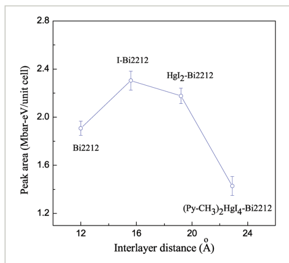
Fig. 2: Hole content in the \text{CuO}_2 planes as a function of interlayer distance between the \text{CuO}_2 planes in adjacent block of pristine Bi2212, I-Bi2212, \text{HgI}_2 -Bi2212, and (\text{Py-CH}_3)_2\text{HgI}_4 -Bi2212.
