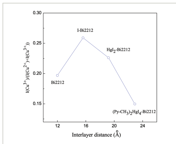
Fig. 4: Normalized intensity, I(\text{Cu}^{3+})/(I(\text{Cu}^{2+})+I(\text{Cu}^{3+})) , as a function of interlayer distance between the \text{CuO}_2 planes in adjacent block of pristine Bi2212, I-Bi2212, \text{HgI}_2 -Bi2212, and (\text{Py-CH}_3)_2\text{HgI}_4 -Bi2212.
