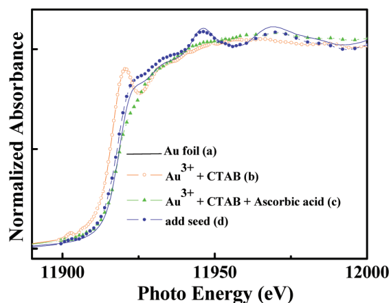
Fig. 2: X-ray absorption spectra of Au L_3 edge during the experiment in the presence of (a) Au foil, (b) prior to adding ascorbic acid, (c) adding ascorbic acid, and (d) adding seed particles, respectively.
