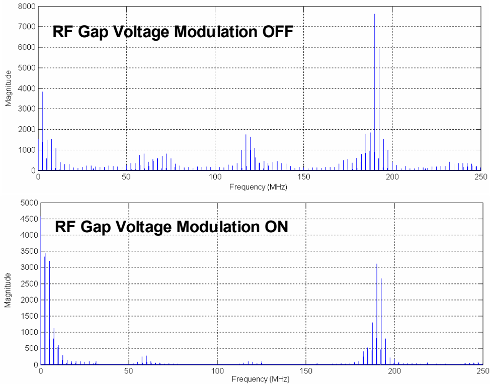
Fig. 5: Longitudinal pseudospectrum of the stored beam with/without RF gap voltage modulation.
