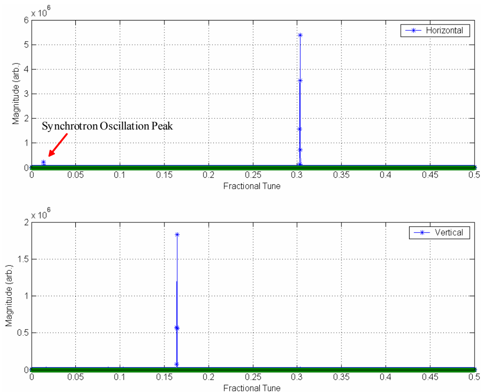
Fig. 8: Tune spectrum obtained from a Fourier analysis of the data set in Fig. 7.
