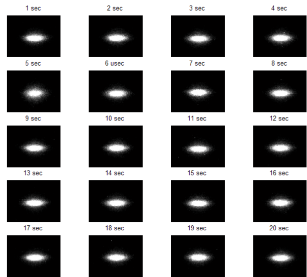
Fig. 4: Single turn profile observation for 20 sec, the storage ring operated with the SRF system. The time on the top of each profile image is the time elapsed after the beginning of image acquisition.
