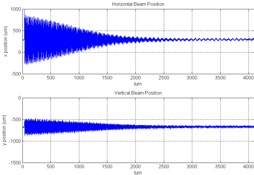
Fig. 7: Turn-by-turn beam position measured using the new digital BPM. The upper figure presents the horizontal beam position, and the lower figure shows the vertical beam position.
