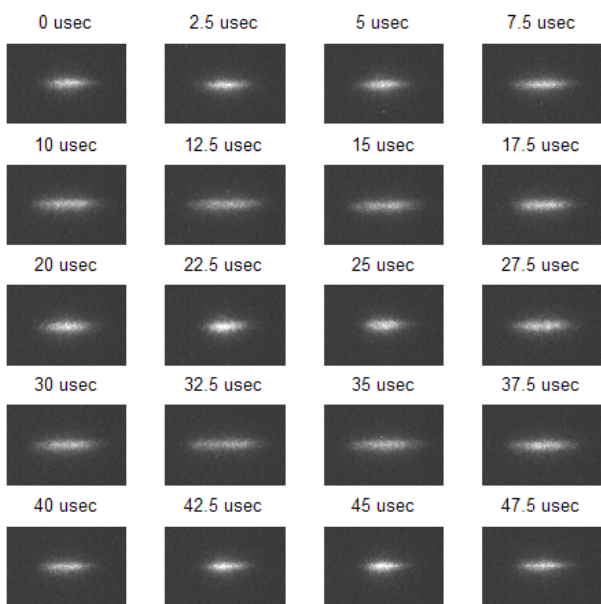
Fig. 3: Single turn beam profile observation to investigate RF gap voltage modulation effects. The image was obtained with a time delay relative to the RF gap voltage modulation signal. The period of the modulation signal is around 20 \mu sec.
