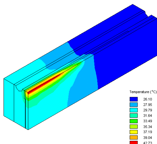
Fig. 2: The simulated temperature distribution of crystal and cooling substrate.
