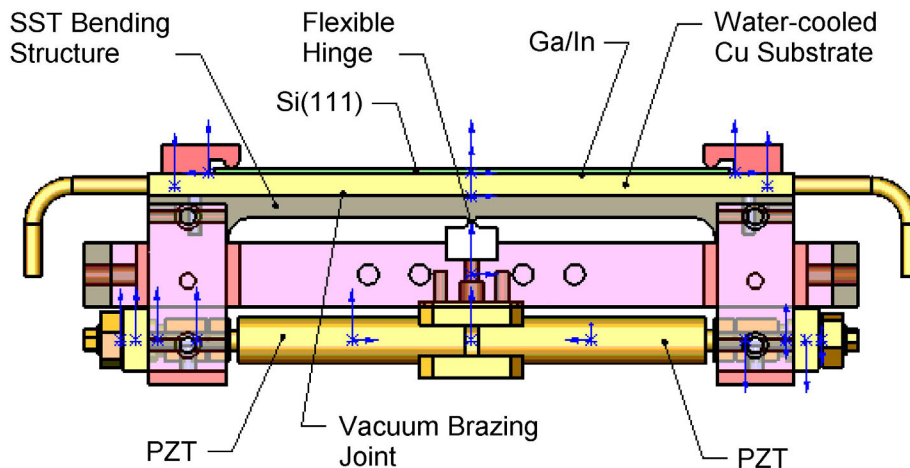
Fig. 1: The bender and cooling mechanism of the curved crystal monochromator.
