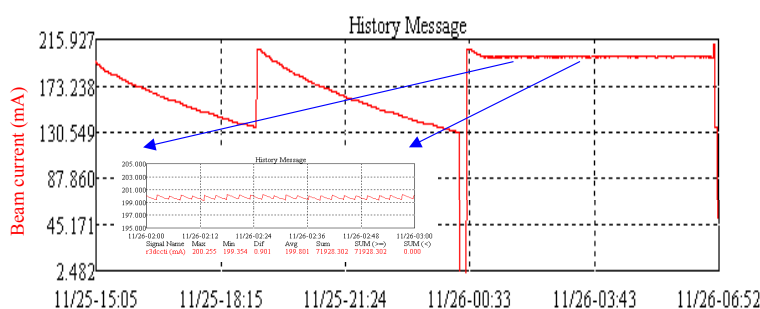
Fig. 1: Stored beam current in decay mode and top-up injection mode and zoom-in the beam current during the top-up injection.
