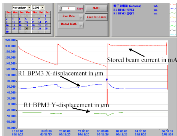
Fig. 2: Recorded structure displacement in vertical and horizontal direction of BPM during decay and top-up injection mode.
