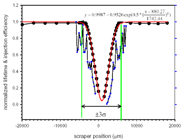
Fig. 3: Vertical scrapers were used to identify the minimum clearance of the ring without affecting the beam lifetime and the injection efficiency.
