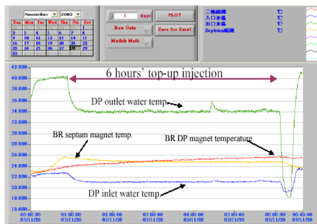
Fig. 4: The temperature readings of dipole magnet and septum core under intermittence operation mode of injector at TLS.
