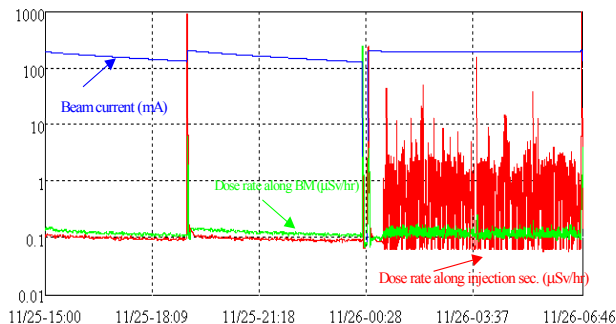
Fig. 5: Stored beam current and dose rate at shielding walls outside of injection section and bending magnet during decay and top-up injection modes.
