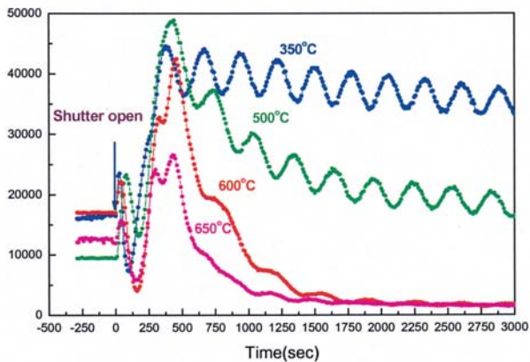
Fig. 2: Real-time measurement of the X-ray intensity at anti-Bragg point (0 0 0.5) of STO on STO deposition by sputtering with different substrate temperatures.
