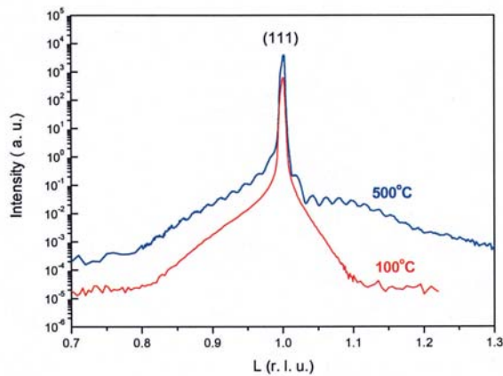
Fig. 6: Profiles of the (111) crystal truncation rod of two LNO films on STO substrates grown at 100 °C and 500 °C.
