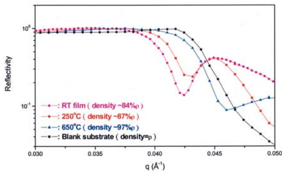
Fig. 5: The detailed profile near total reflection angle of X-ray reflectivity curves for different STO films.
