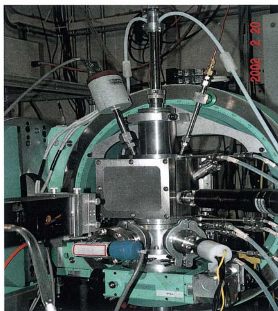
Fig. 1: The oxide growth chamber mounted on a Huber 8-circle diffractometer.
