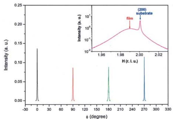
Fig. 4: The azimuthal scan around the surface (200) peak of a STO film deposited at 750°C. Inset: In-plane diffraction profile of (200) reflection.
