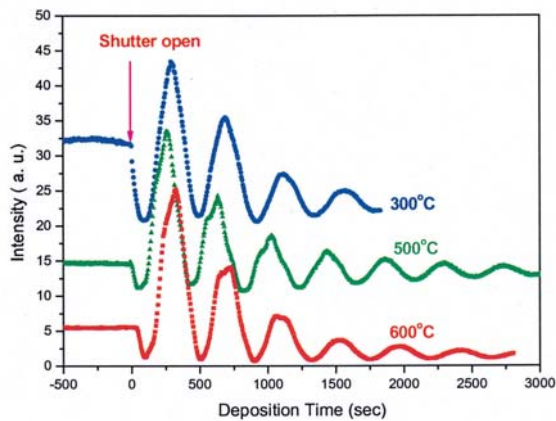
Fig. 3: Real-time intensity oscillations at (0 0 0.75) of LNO on STO substrate during RF sputtering with different substrate temperatures.
