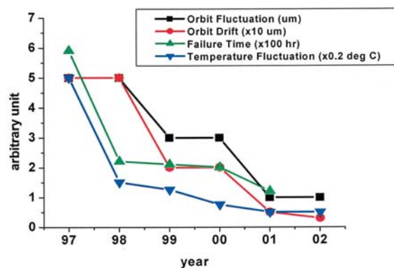
Fig. 2: Performance improvements of TLS from 1997 to 2002.
