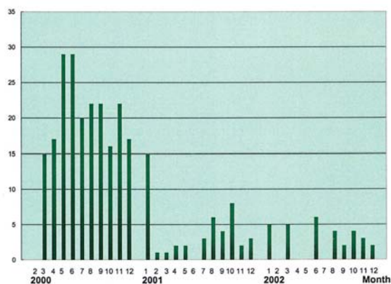
Fig. 3: Number of beam loss per month from 2000 to 2002. The performance in year 2000 was abnormal due to some coincidental problems.
