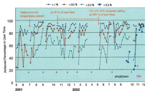
Fig. 4: Instability index ( \Delta/I ) from May 2001 to December 2002.
