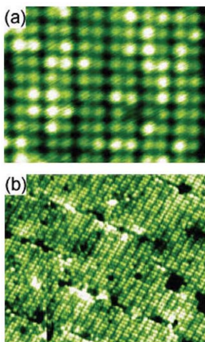
Fig. 1: STM images obtained with a tunneling current of 0.05 nA and a sample bias of 1.9 V. (a) is for Si(100) after one cycle of Ge ALE growth and Cl termination, and covers an area of 48 \times 36 \text{ \AA}^2 . The bright and dark atoms correspond to Cl adsorbed on Ge and Si, respectively. (b) is the same but for two cycles of Ge ALE growth and an imaged area of 205 \times 165 \text{ \AA}^2 .
