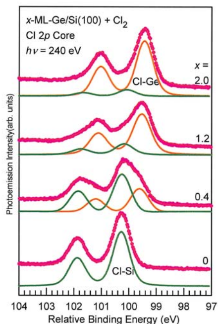
Fig. 3: Photoemission spectra for the Cl 2p core level. The samples are Cl-terminated Si deposited with 0, 1, 3, and 5 cycles of Ge ALE (corresponding to Ge deposition of 0, 0.4, 1.2, and 2.0 ML, respectively). The two components, Cl-Si and Cl-Ge, correspond to Cl bonded to Si and Ge, respectively.
