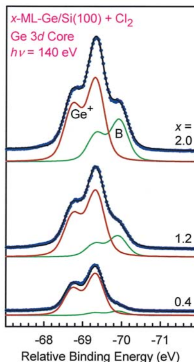
Fig. 4: Photoemission spectra for the Si 2p and Ge 3d core levels. The samples are Cl-terminated Si deposited with 0, 1, 3, and 5 cycles of Ge ALE (corresponding to Ge deposition of 0, 0.4, 1.2, and 2.0 ML, respectively). Two components are seen in each case. The components labeled Si + and Ge + correspond to Si and Ge dimer atoms directly bonded to Cl, respectively, while the B components correspond to Si and Ge in the subsurface region.
