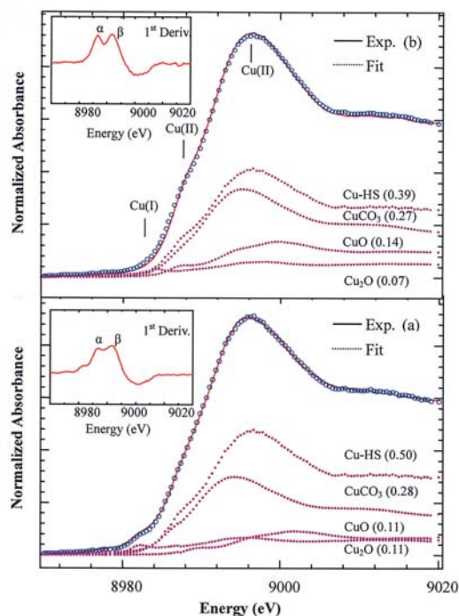
Fig. 2: Experimental data (solid line) and the least-square fits (circles) for the XANES spectra of the Cu-contaminated soil (a) before and (b) after 180 min of EKR. Dotted lines denote fractional contributions of the four main copper species making up the fitted spectra.
