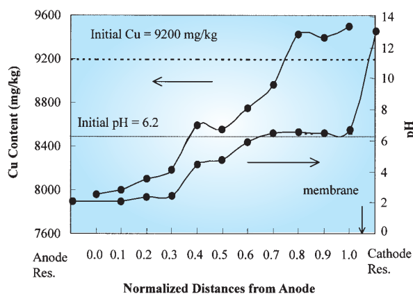
Fig. 1: Copper concentration and pH profile across soil after 180 min of the EKR.
