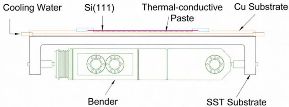
Fig. 2: Schematic drawing of the bending and cooling mechanisms of ACCM.
