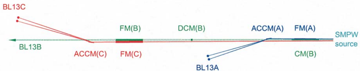
Fig. 1: Top view of the optical layout of the central and side-branch beamlines, which share the output of the Superconducting Multipole Wiggler (SMPW) source. ACCM: Asymmetric-cut Curved Crystal Monochromator. DCM: Double Crystal Monochromator. CM: Collimating Mirror, FM: Focusing Mirror.
