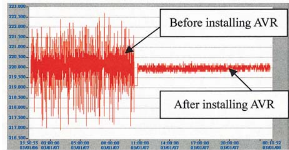
Fig. 3: The AC line voltage, supplied to the Q4 power supply, before and after using a precision voltage regulator of 300kVA.
