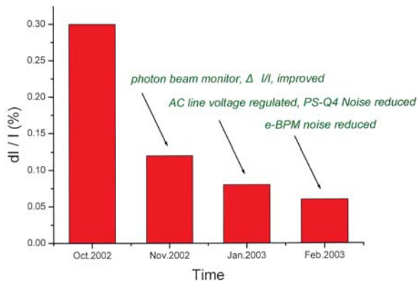
Fig. 2: Reductions in the photon beam fluctuation in 2002-2003.
