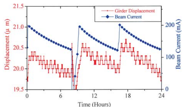
Fig. 1: The correlation between beam current and girder displacement.
