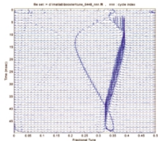
Fig. 10: Tune variation during energy ramping.
