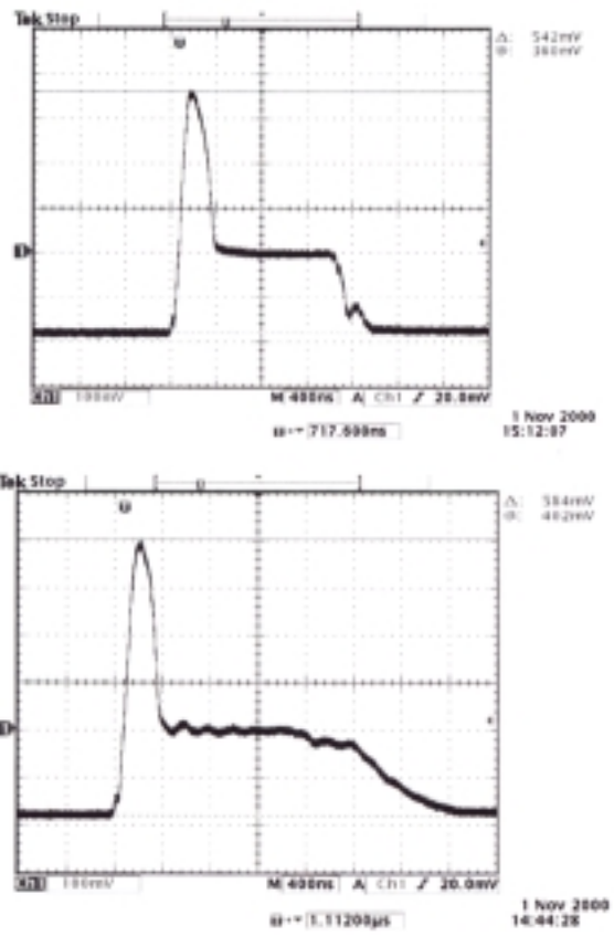
Fig. 6: (a) High voltage pulse signal measured at grid 2 of CX1159 with DEI-100 pulser. (b) High voltage pulse signal measured at grid 2 of CX1159 with SRRC-1000. (Scale : 1V=1000V)
