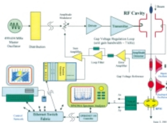
Fig. 8: Setup of the gap voltage modulation experiment.
