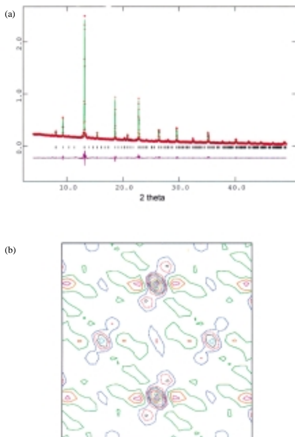
Fig. 2: X-ray powder diffraction results obtained from Ba_2HoRu_{0.9}Cu_{0.1}O_6 with a curved image plate: (a) X-ray powder pattern; (b) charge density.
