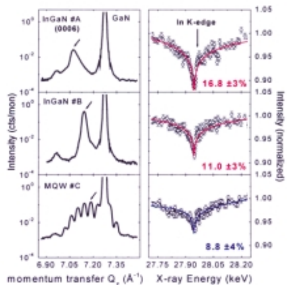
Fig. 3: Anomalous X-ray scattering profiles measured at Bragg peak (0 0 6) across In K-edge for two single-quantum well samples (samples # A and B) and a multiquantum-well sample. The depth of the intensity cusp is very sensitivity to the indium composition.
