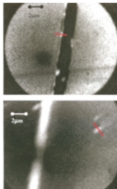
Fig. 3: (a) The image of the Pd/Si sample taken with Hg light. The signal from the Pd stripes is hardly measurable, because the work function of generating secondary electron from Pd is higher than the energy provided by the Hg light. The best spatial resolution obtained in this image is 0.1 \mu m. (b) The image of the Pd/Si sample taken with SR light. The signal from the Pd stripes is higher than that from the Si substrate at h\nu = 130 eV. The best spatial resolution obtained in this image is 0.18 \mu m. The dark area located at lower left part of both images shows the low efficiency of the MCP, which may be damaged.
