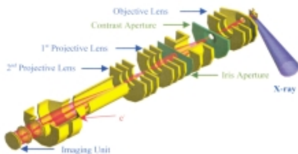
Fig. 1: Cartoon presentation of PEEM optics and electron path.
