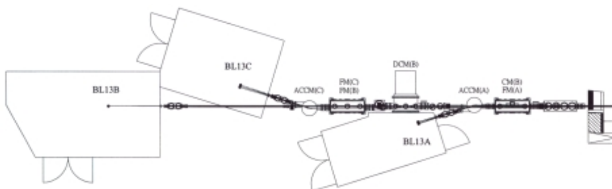
Fig. 2: The layout of the biological crystallography beamlines BL13A, BL13B and BL13C.
