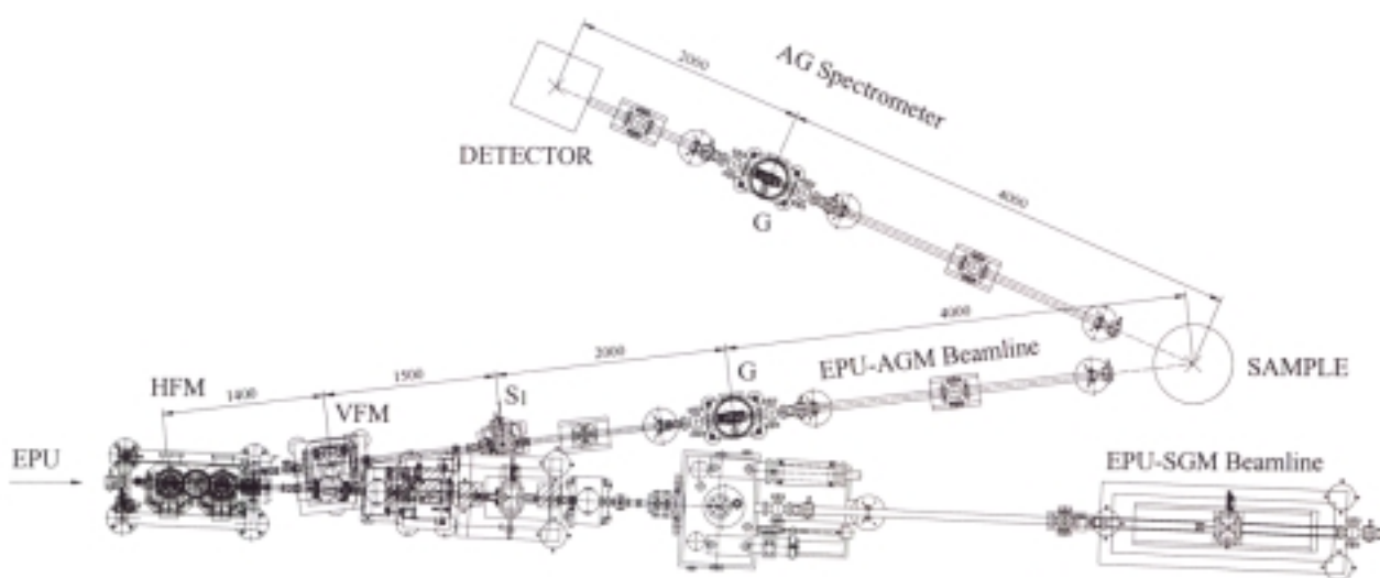
Fig. 3: The layout of EPU-AGM beamline and AG spectrometer.
