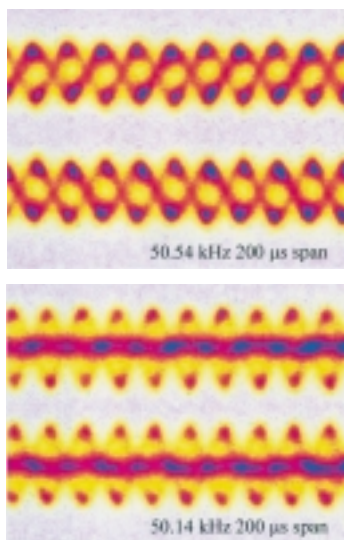
Fig. 3: Longitudinal motion of multi-bunch beam under rf amplitude modulation. The modulation frequencies were 50.54 kHz for the top graph and 50.14 kHz for the bottom graph. The modulation amplitude was 2.6% of the rf voltage. The full vertical was 1.4 ns and the horizontal scale was 200 \mu s. Note that the modulation frequency of the top graph was within f_{bif-} and f_{bif+} , and thus there existed only two beamlets. Since the modulation frequency in the bottom graph was below f_{bif-} , there were three beamlets in the bucket.
