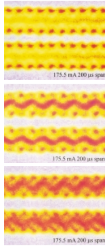
Fig. 1: Collective beam instability observed from images of streak-camera at 175.5 mA without rf voltage modulation. The images have a total time-span of 200 \mu s taken randomly at different time for an identical machine operational condition. The graphs taken at different times show different characteristic behaviors.
