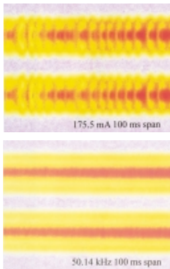
Fig. 2: The images of streak camera in a time-span of 100 ms. When rf voltage modulation with frequency 50.14 kHz was applied to the beam shown in the top graph, the beam became stable as shown in the bottom graph. This image corresponds to three beamlets rotate around the center of the bucket. See the bottom graph of Fig. 3 for a smaller time-span of 200 \mu s.
