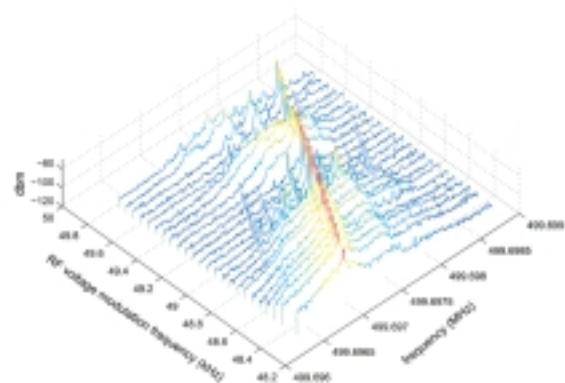
Fig. 7: The observed 2 f_s synchrotron sideband power spectrum (in the unit of dBm) for a sum signal in the peak-hold mode for the TLS at 190 mA, nearly uniformly distributed in 160 bunches. Note that the 2 f_s sideband induced by wake field is highly suppressed when the modulation frequency was about 49.2 kHz.
