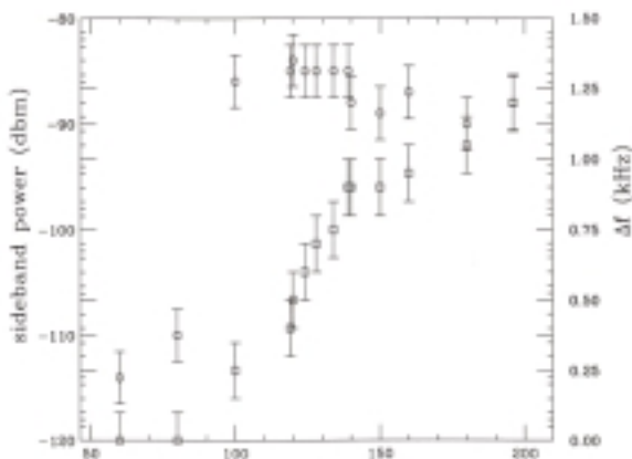
Fig. 6: The peak power of 2 f_s (circles) and the width \Delta f = f_{bif+} - f_{bif-} (rectangles) are shown as a function of the beam current. Note that the threshold current for the instability is about 100 mA.
