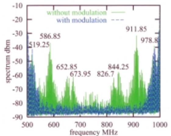
Fig. 4: Beam spectrum from BPM sum signal before and after applying rf voltage modulation. The modulation frequency was 50.155 kHz and the amplitude of modulation was 3.1%. The frequency span of the spectrum was 500 MHz.
