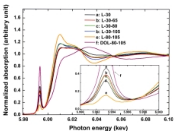
Fig. 3: Cr XANES spectra for mildly heated samples. The pre-edge features have been magnified in the inset for clarity.
