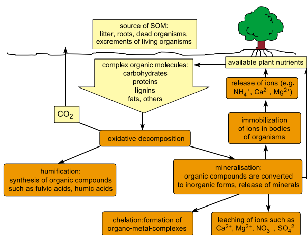
Fig. 1: Transformation of soil organic matters within soil. Courtesy of Prof. S. Grunwald, U. of Florida, at a website address of http://grunwald.ifas.ufl.edu .
